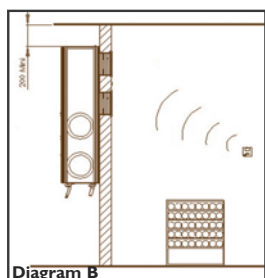
Conditioner housed outside the cellar with extraction on the left side / aesthetic front panel on the inside.
